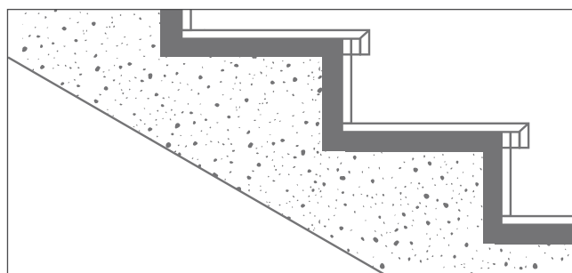
GRADONE CON RANURAS STEP TREAD (REINFORCED OVER-HANGING) WITH GROOVES
